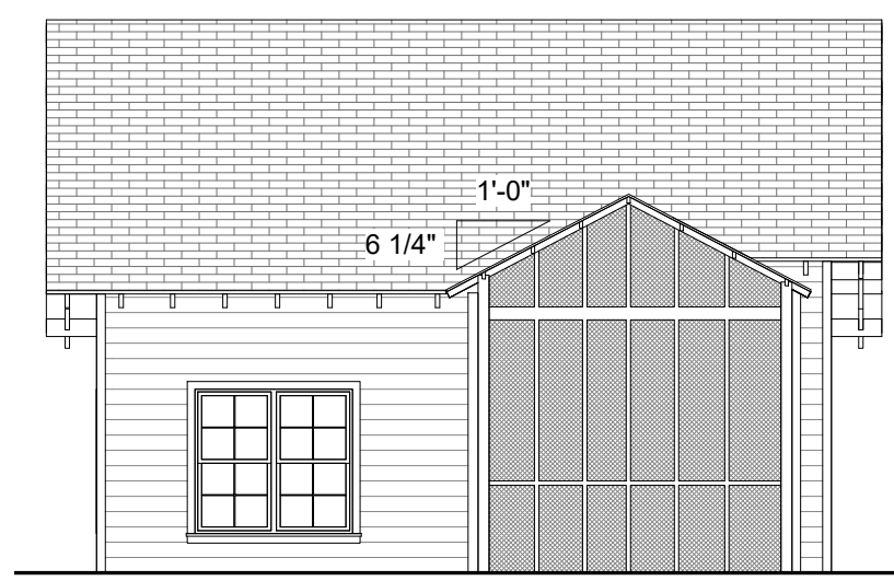
① NORTH ELEVATION 1/8" = 1'-0"
