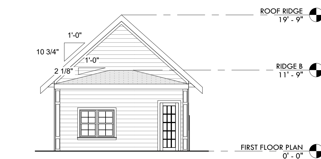
1 NORTH ELEVATION 1/8" = 1'-0"
