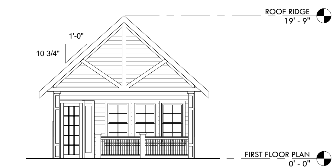
3 SOUTH ELEVATION 1/8" = 1'-0"
